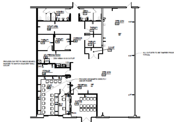
2 POWER/DATA LOCATION PLAN SCALE: 1/8" = 1'-0"
